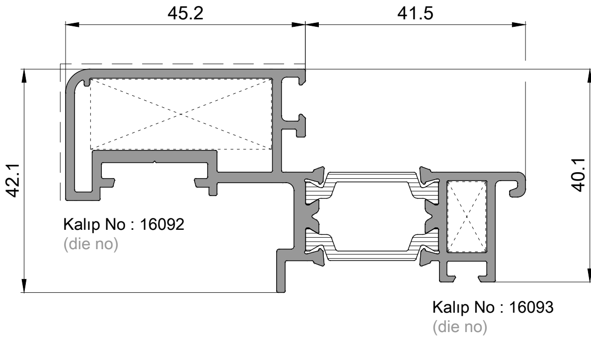
P 2508 Kanat Profili / Sash Profile 1,490kg/mt
