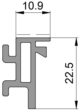
P 2515 Adaptor Profili / Adepter Profile 0,320kg/mt
