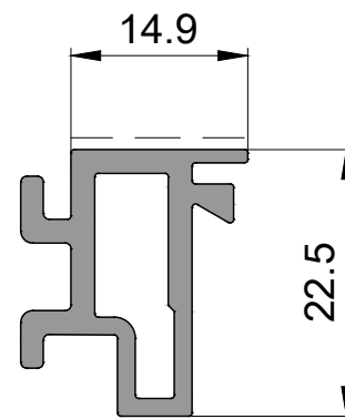
P 2514 Adaptor Profili / Adepter Profile 0,400kg/mt
