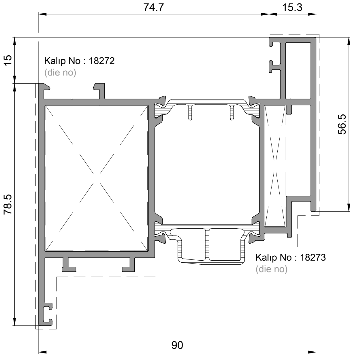
P 2196 Kanat Profili / Sash Profile 2,445kg/mt
