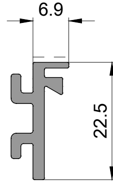
P 2516 Adaptor Profili / Adepter Profile 0,250kg/mt
