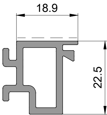
P 2513 Adaptor Profili / Adepter Profile 0,470kg/mt
