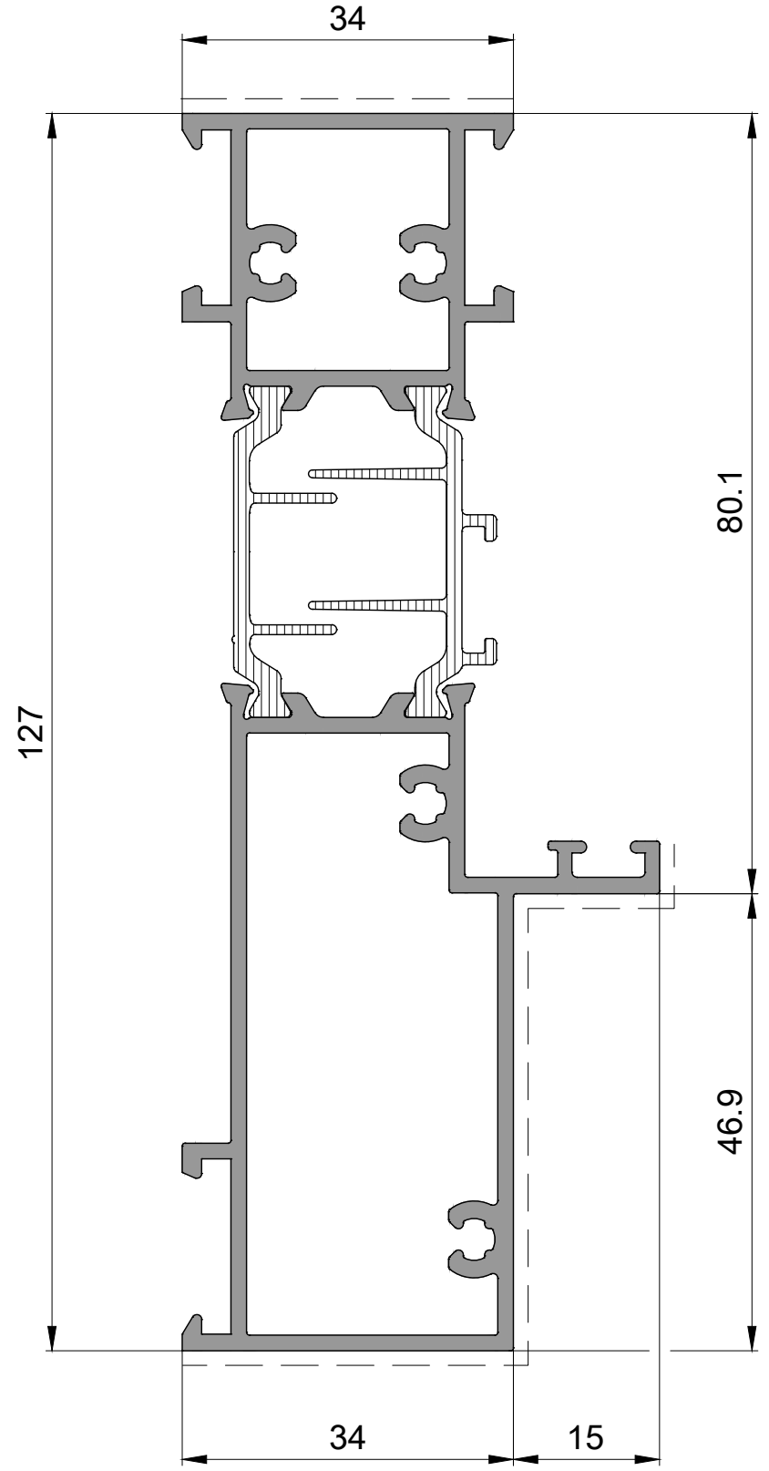
P 2504 Yatay Profil / Transom Profile 2,160kg/mt
