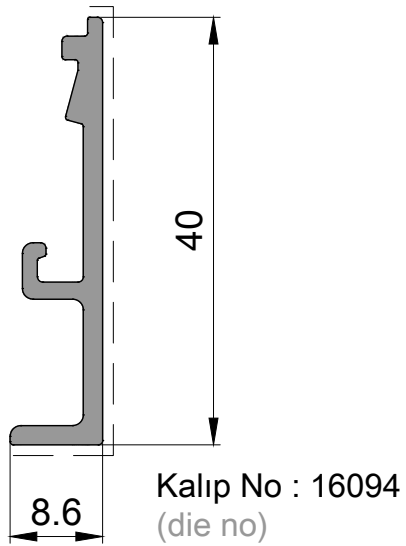
P 1699 Cam Çıta Profili / Glazing Bead Profile 0,300kg/mt
