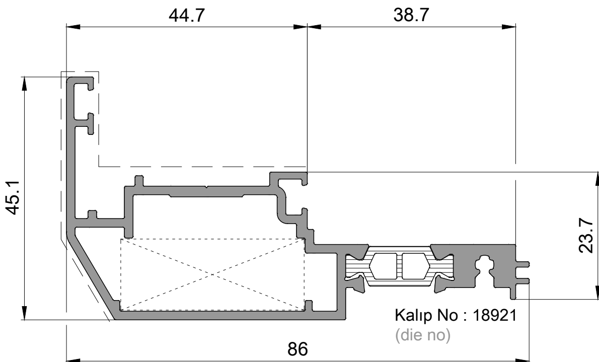
P 2510 Kasa Profili / Frame Profile 1,245kg/mt
