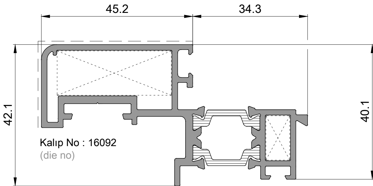
P 2509 Kanat Profili / Sash Profile 1,450kg/mt
