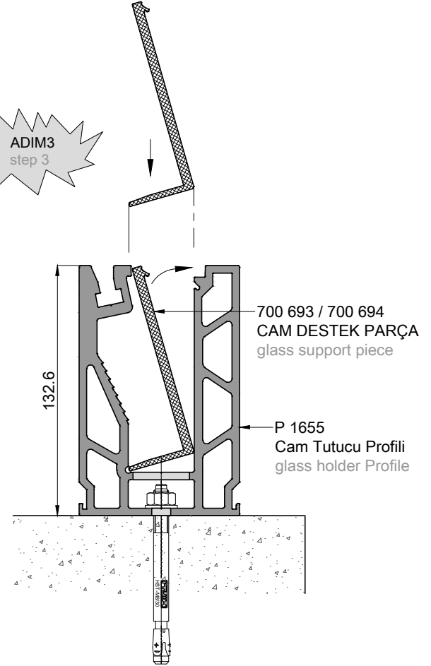
700 693 / 700 694 CAM DESTEK PARÇA glass support piece
