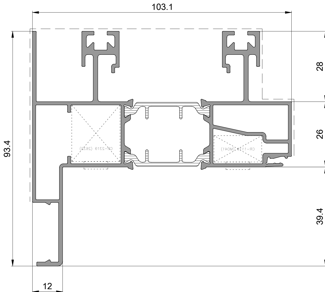
P 2586 Alt Kasa Profili Bottom Frame Profile 2,390kg/mt
