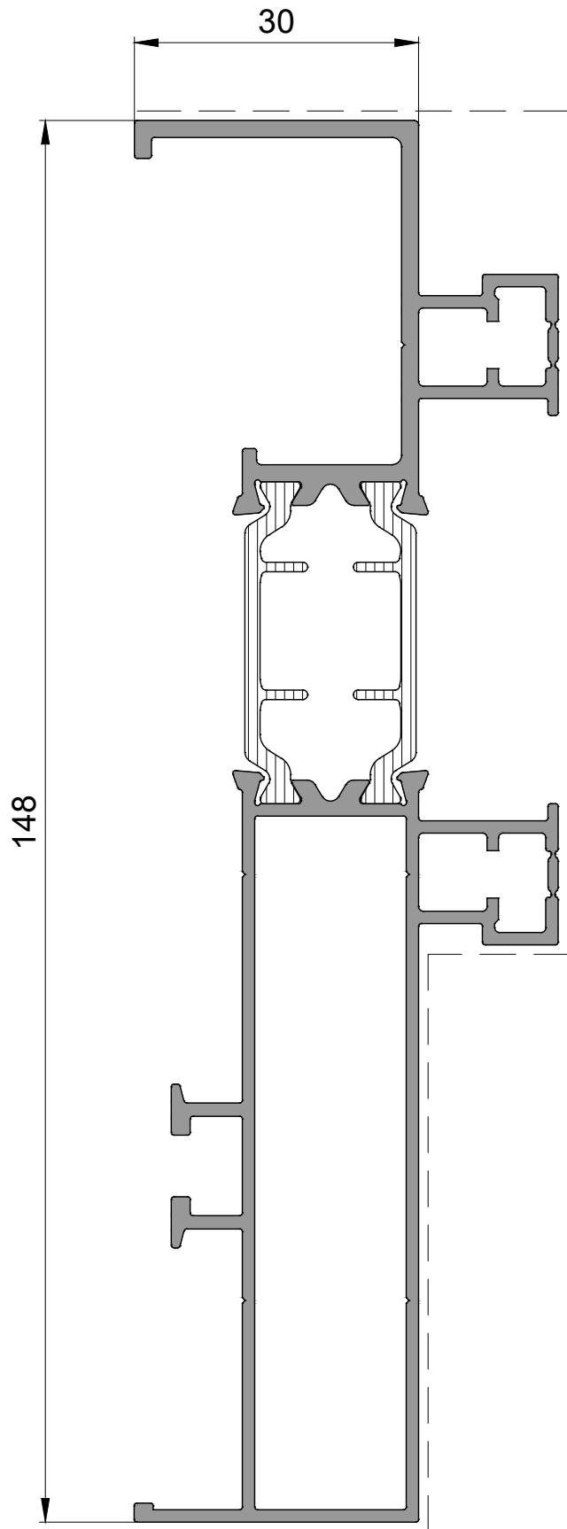
P 2583 Yan Kasa Profili Side Frame Profile 1,885kg/mt
