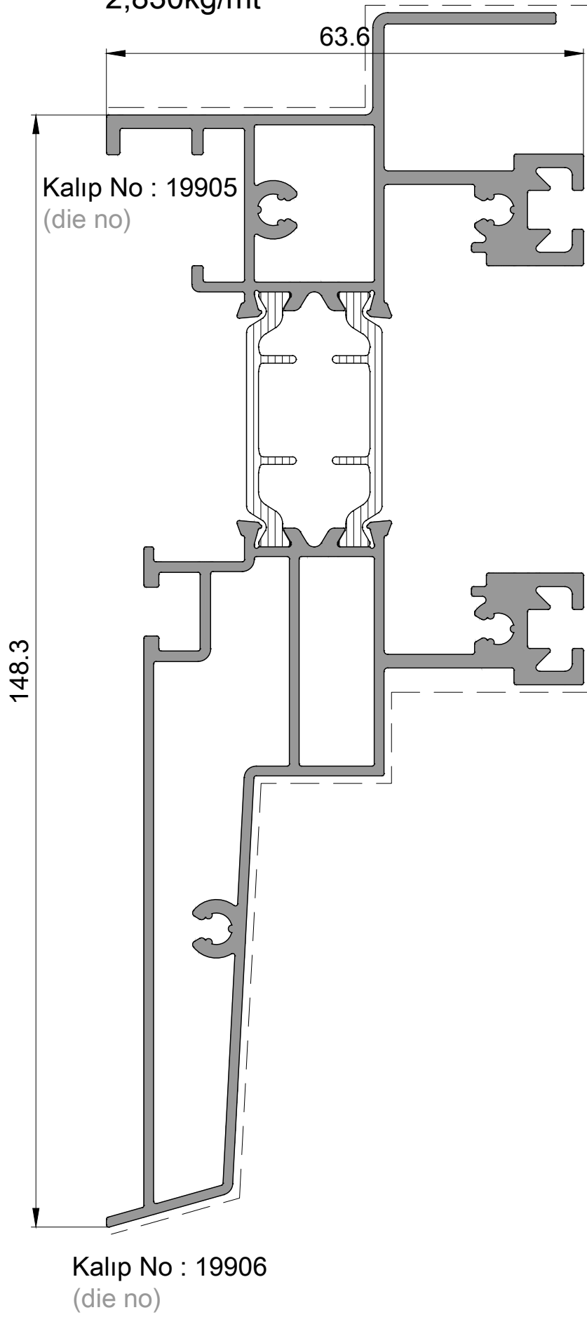
P 2567 Alt Kasa Profili Bottom Frame Profile 2,830kg/mt
