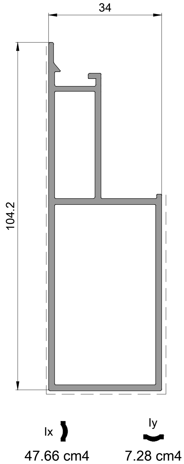
P 2554 Yan Kasa Profili Side Frame Profile 1,335kg/mt
