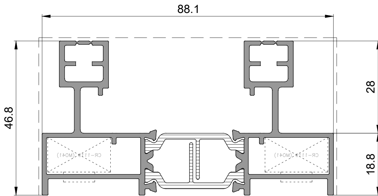
P 2589 Yan Kasa Profili Side Frame Profile 1,650kg/mt
