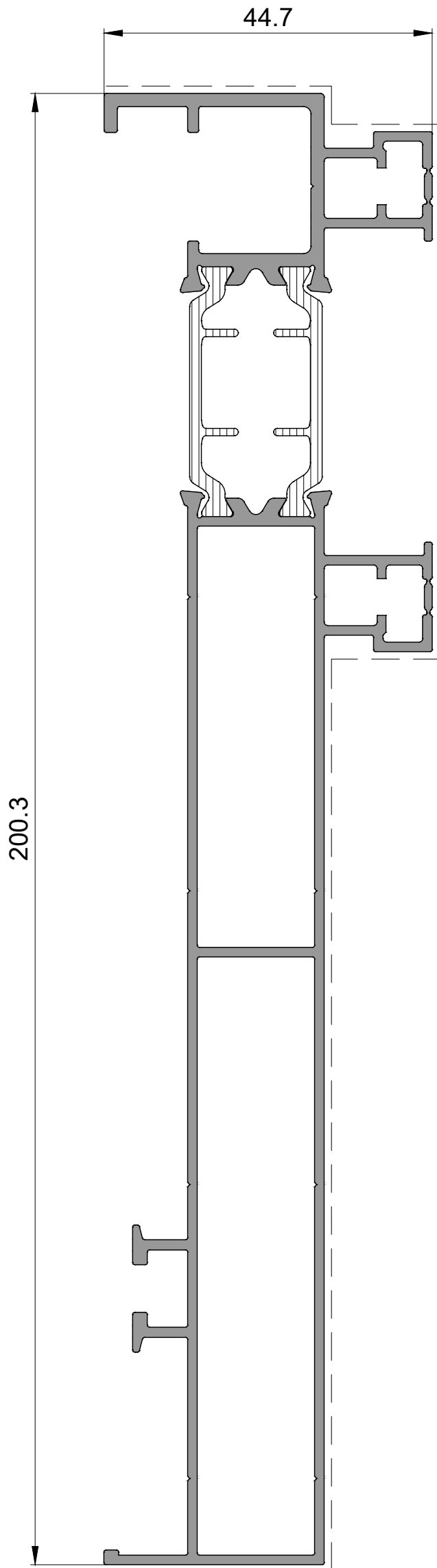
P 2563 Yan Kasa Profili Side Frame Profile 2,360kg/mt
