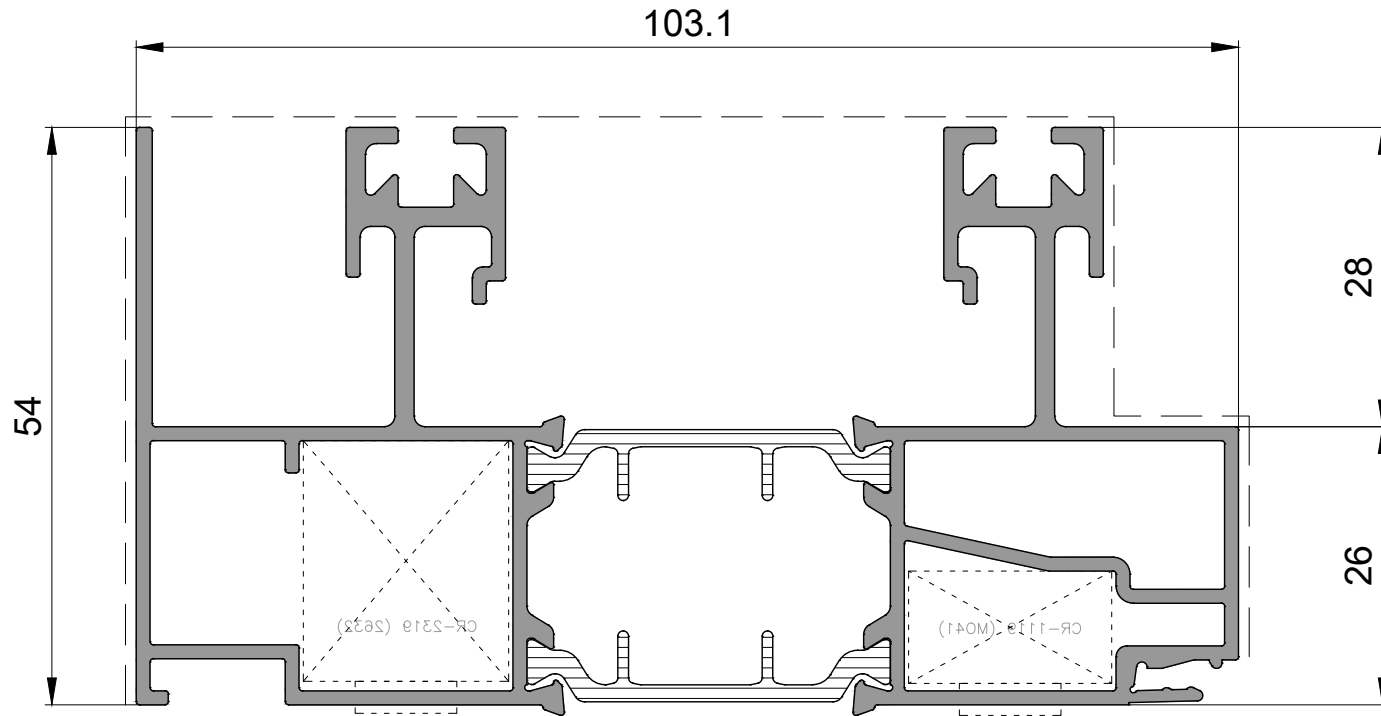
P 2587 Alt Kasa Profili Bottom Frame Profile 2,150kg/mt
