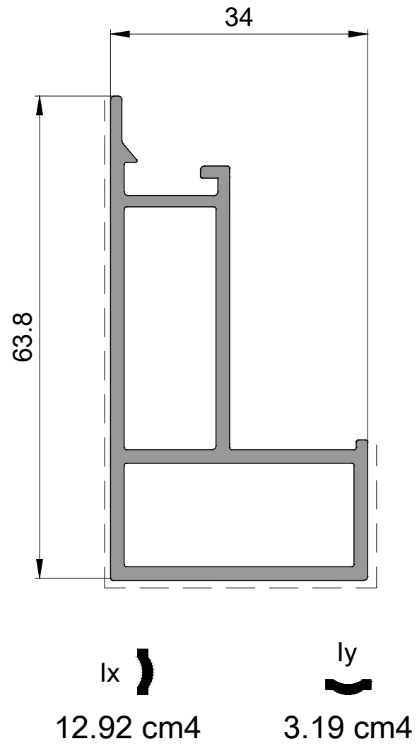
P 2552 Yan Kasa Profili Side Frame Profile 0,940kg/mt
