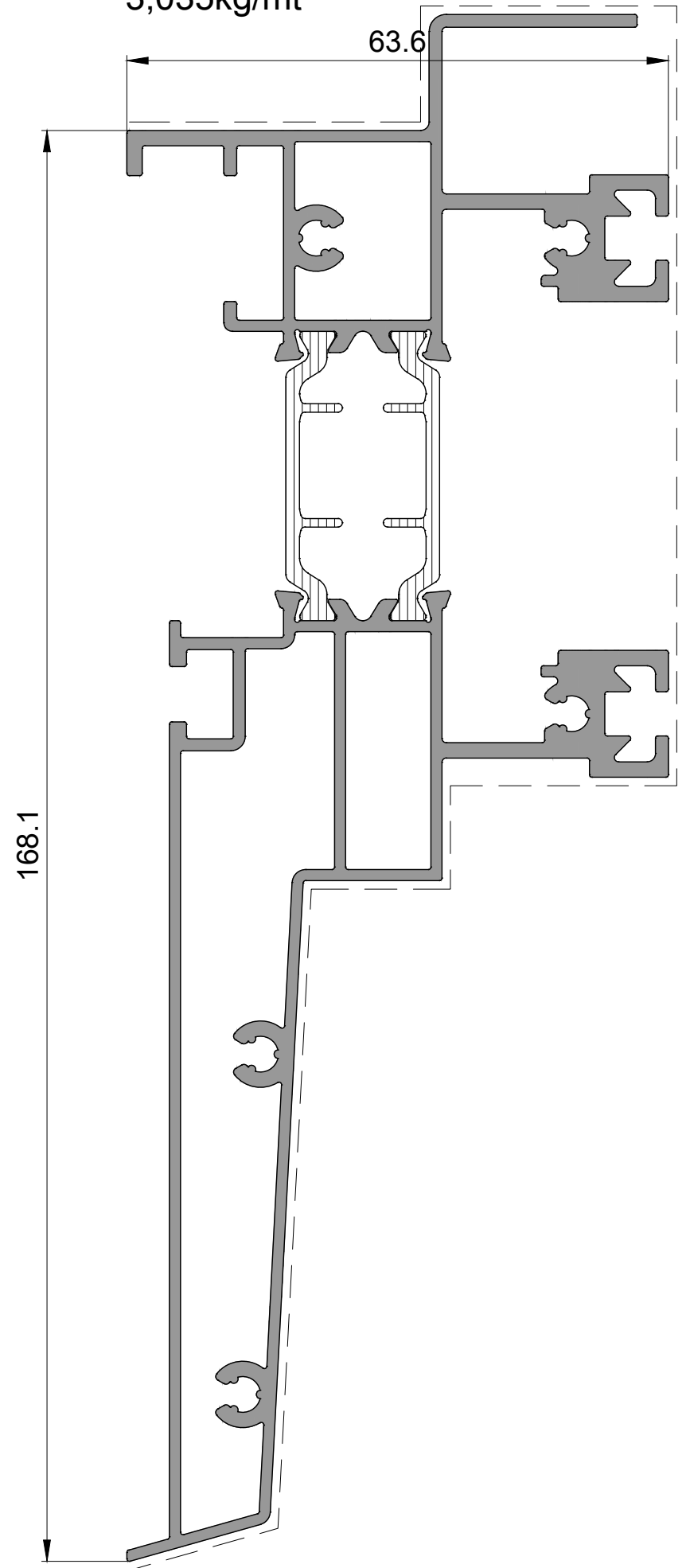
P 2568 Alt Kasa Profili Bottom Frame Profile 3,035kg/mt
