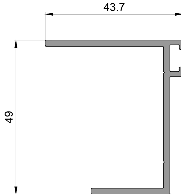
P 2559 Kapatma Profili Closing Profile 0,640kg/mt
