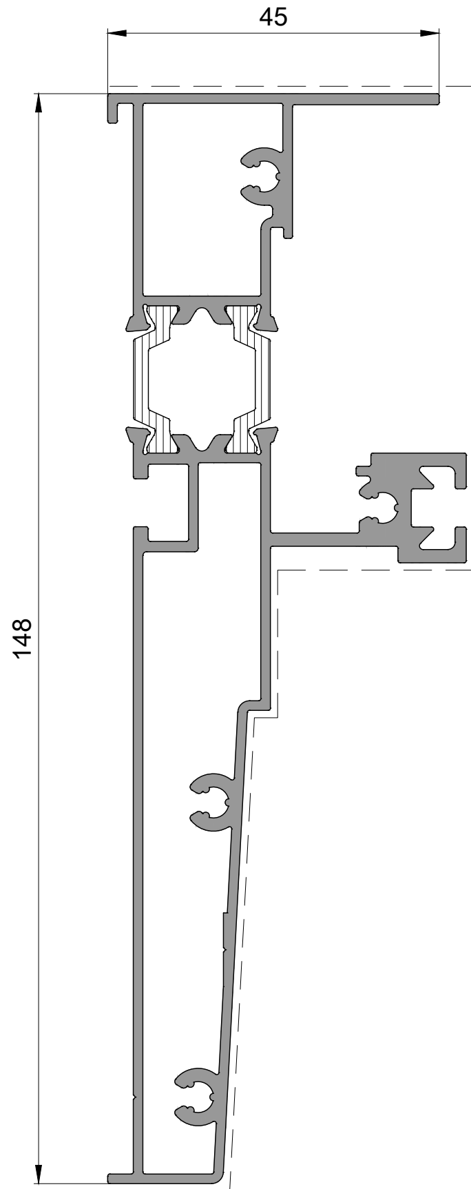
P 2580 Alt Kasa Profili Bottom Frame Profile 2,195kg/mt
