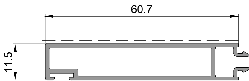
P 2560 Kapatma Profili Closing Profile 0,535kg/mt
