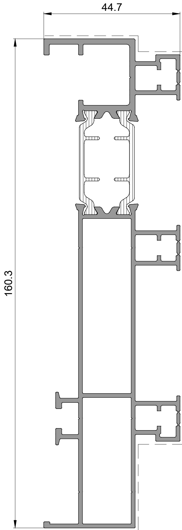
P 2569 Yan Kasa Profili Side Frame Profile 2,235kg/mt
