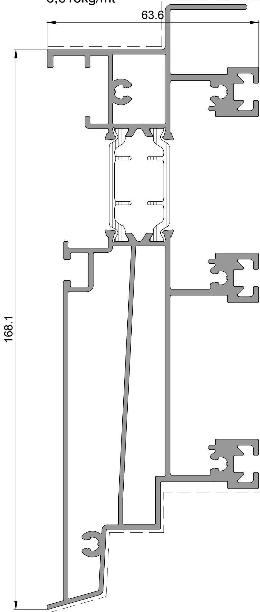
P 2573 Alt Kasa Profili Bottom Frame Profile 3,615kg/mt
