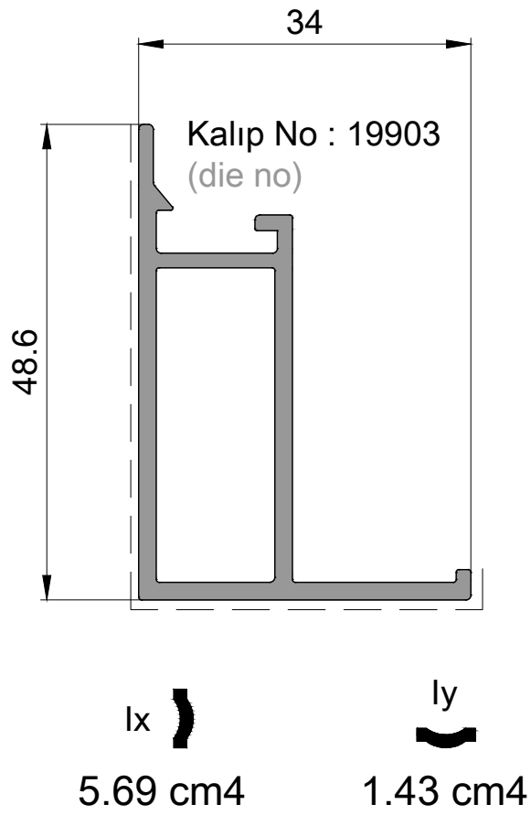
P 2551 Yan Kasa Profili Side Frame Profile 0,640kg/mt
