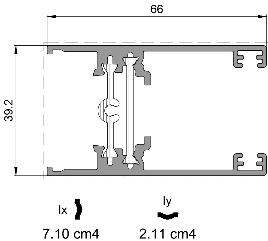
P 2550 Yan Kasa Profili Side Frame Profile 1,280kg/mt
