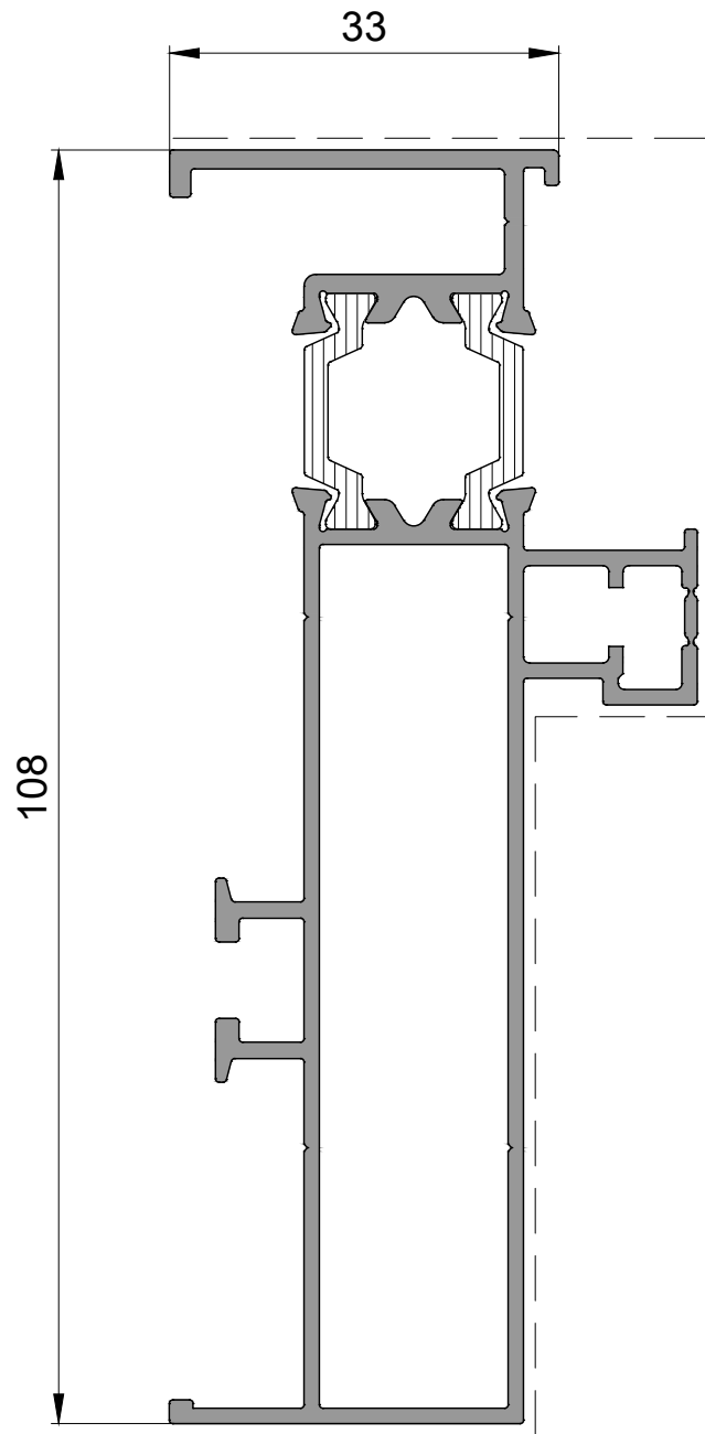
P 2575 Yan Kasa Profili Side Frame Profile 1,510kg/mt
