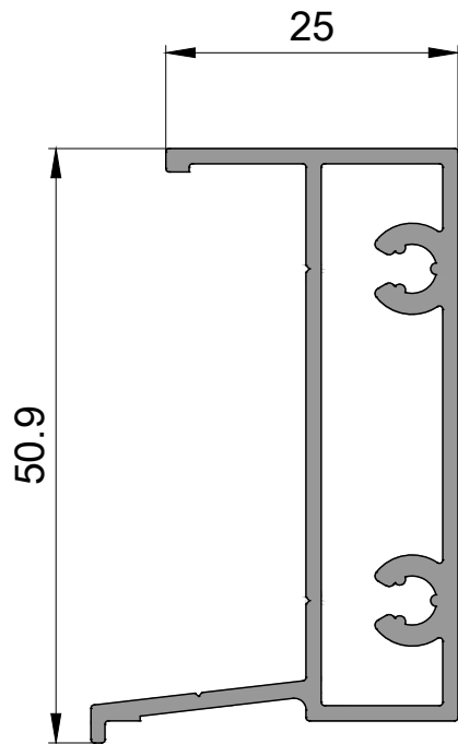
P 2558 Kapatma Profili Closing Profile 0,675kg/mt
