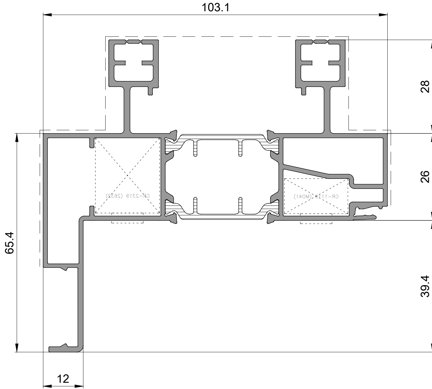
P 2585 Yan Kasa Profili Side Frame Profile 2,205kg/mt
