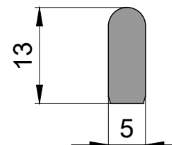
P 2488 Ray Profili / Rail Profile 0,170kg/mt
