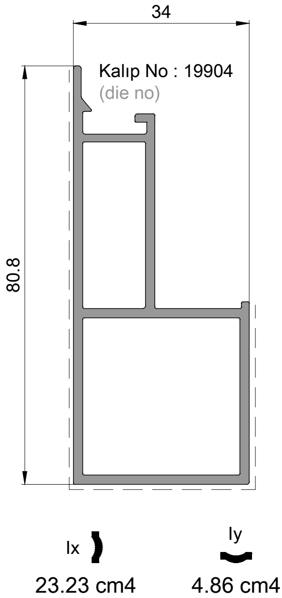
P 2553 Yan Kasa Profili Side Frame Profile 1,105kg/mt
