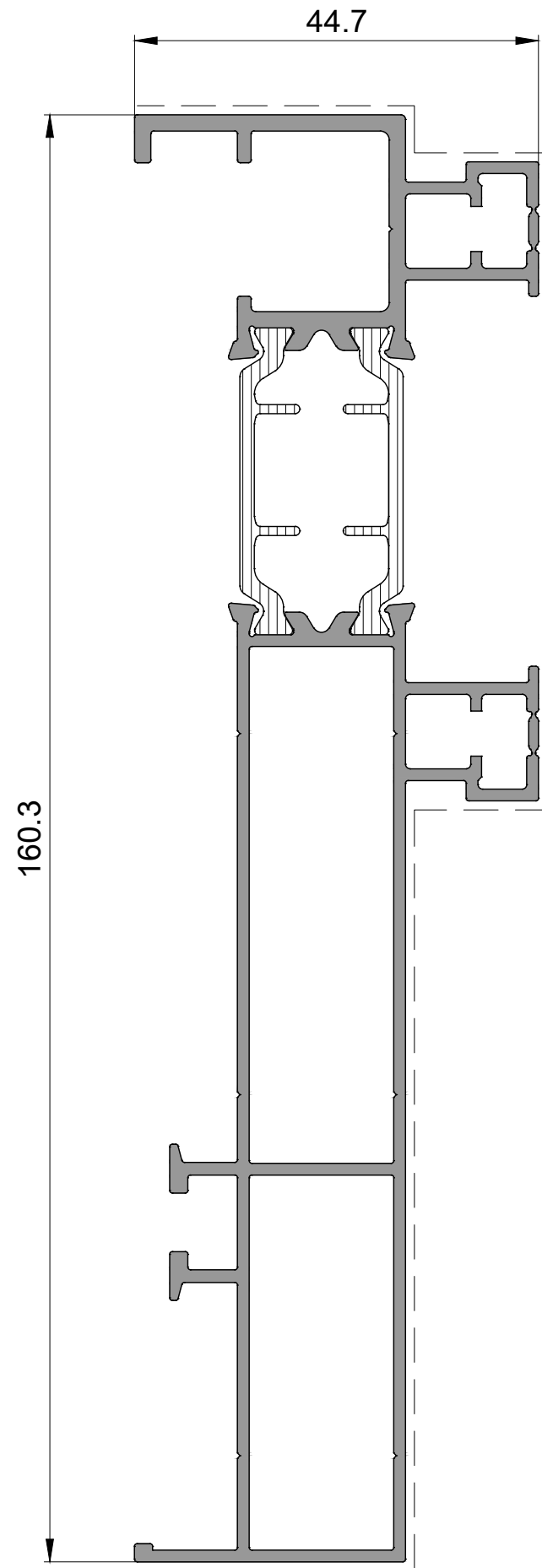
P 2562 Yan Kasa Profili Side Frame Profile 2,080kg/mt
