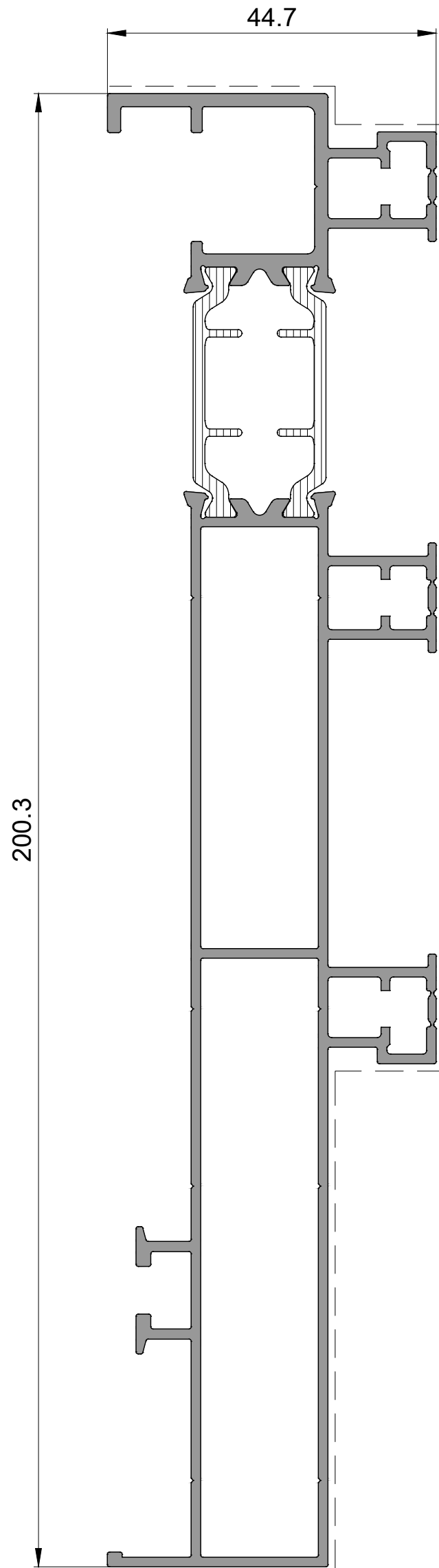
P 2570 Yan Kasa Profili Side Frame Profile 2,515kg/mt
