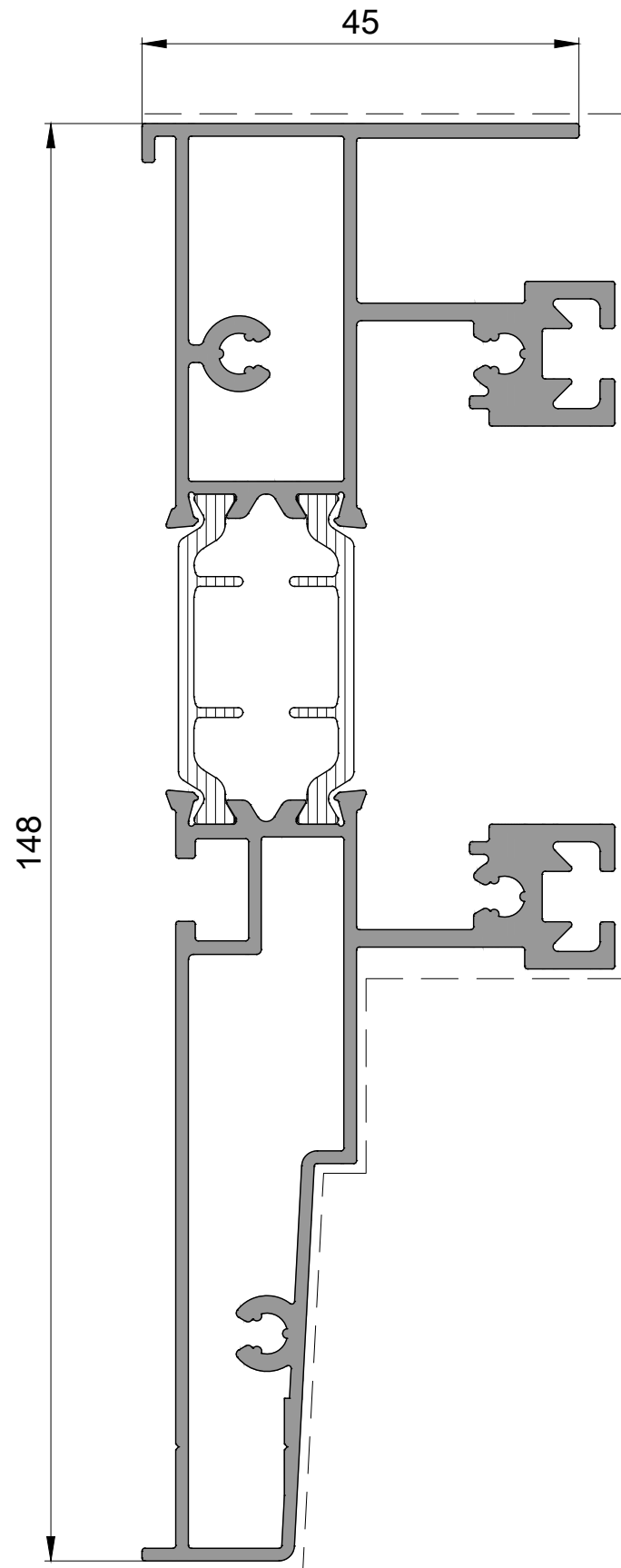
P 2584 Alt Kasa Profili Bottom Frame Profile 2,490kg/mt
