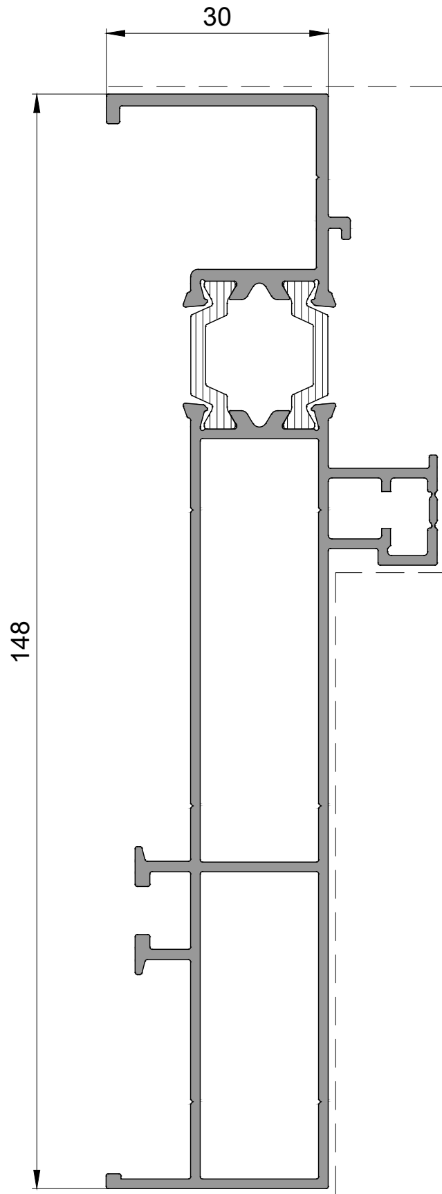
P 2579 Yan Kasa Profili Side Frame Profile 1,810kg/mt
