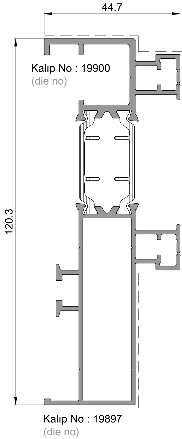
P 2561 Yan Kasa Profili Side Frame Profile 1,740kg/mt
