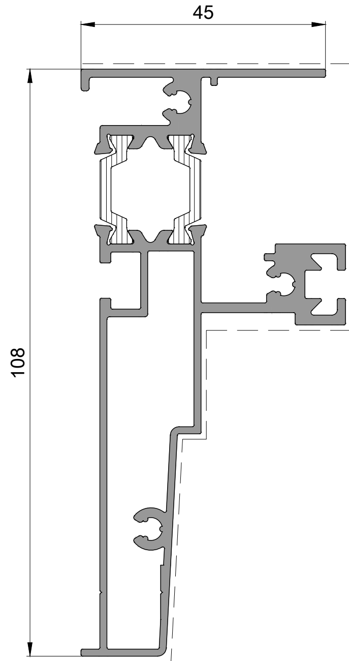
P 2576 Alt Kasa Profili Bottom Frame Profile 1,855kg/mt
