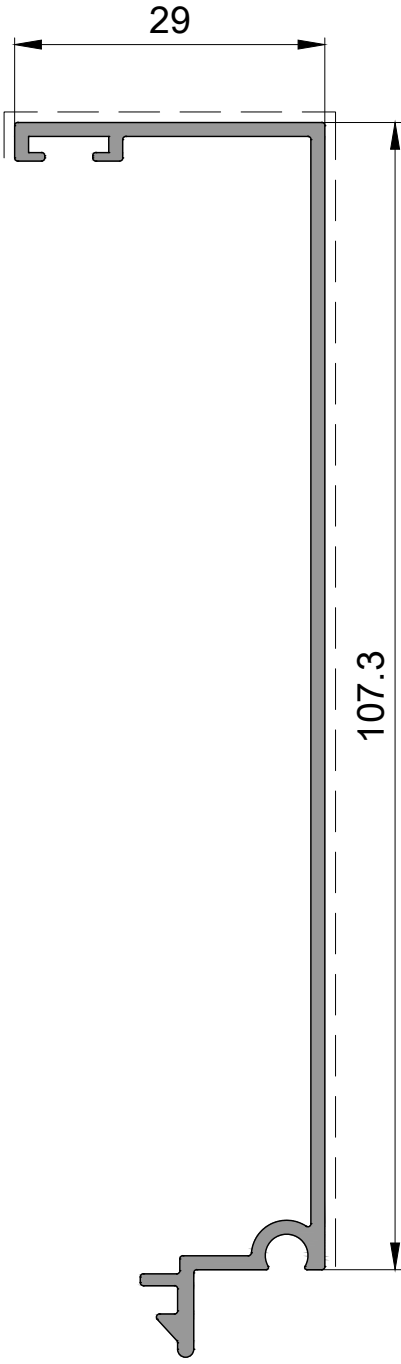
P 2632 Pervaz Profili / Tape Isolation 0,605kg/mt
